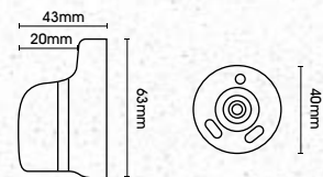
Recess Bracket
