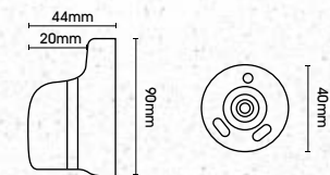
Recess Bracket
