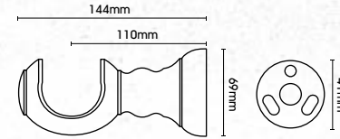
Cup Bracket
